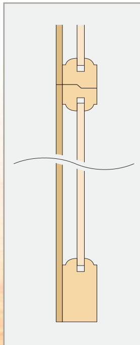
Flat panel door construction detail
