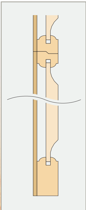
Raised panel door construction detail
